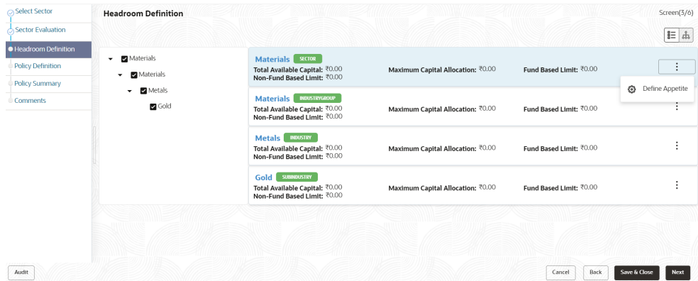
Figure 3-15 Define Appetite
