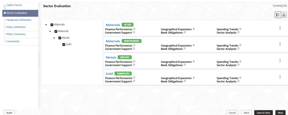
Figure 3-12 Sector Evaluation
