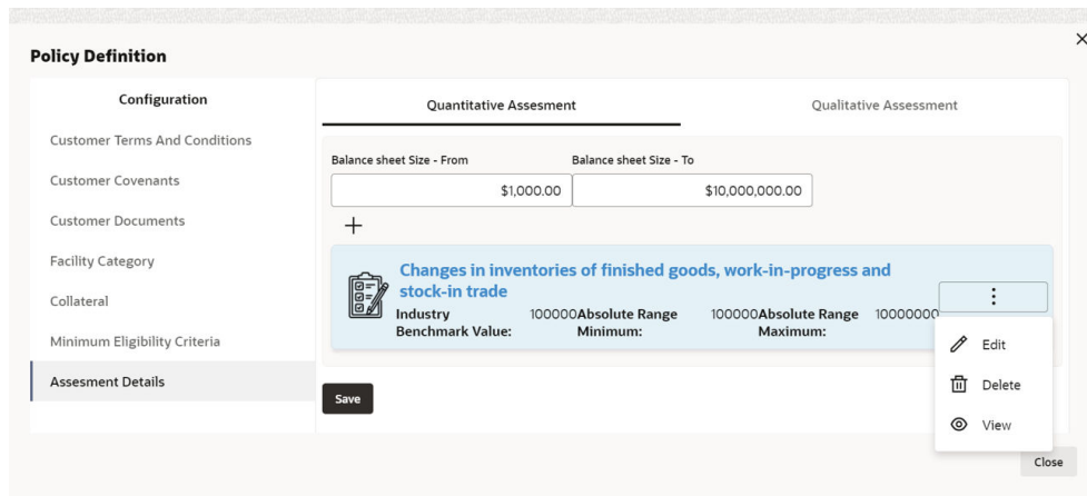
Figure 3-59 Quantitative Assessment
