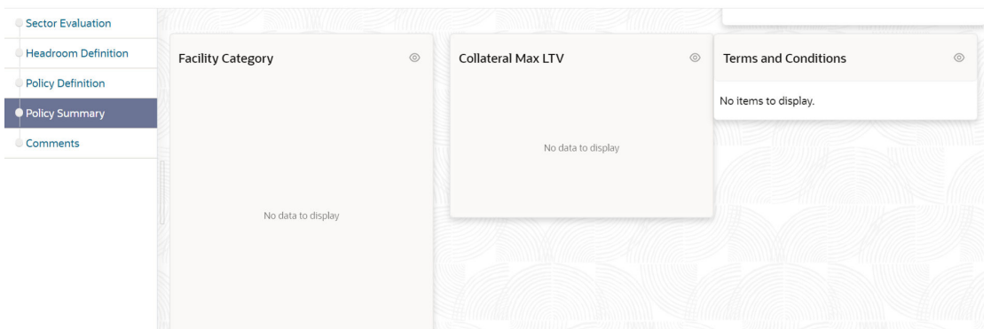
Figure 3-66 Policy Summary
