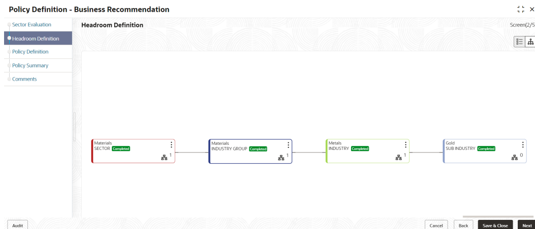
Figure 4-4 Headroom Definition
