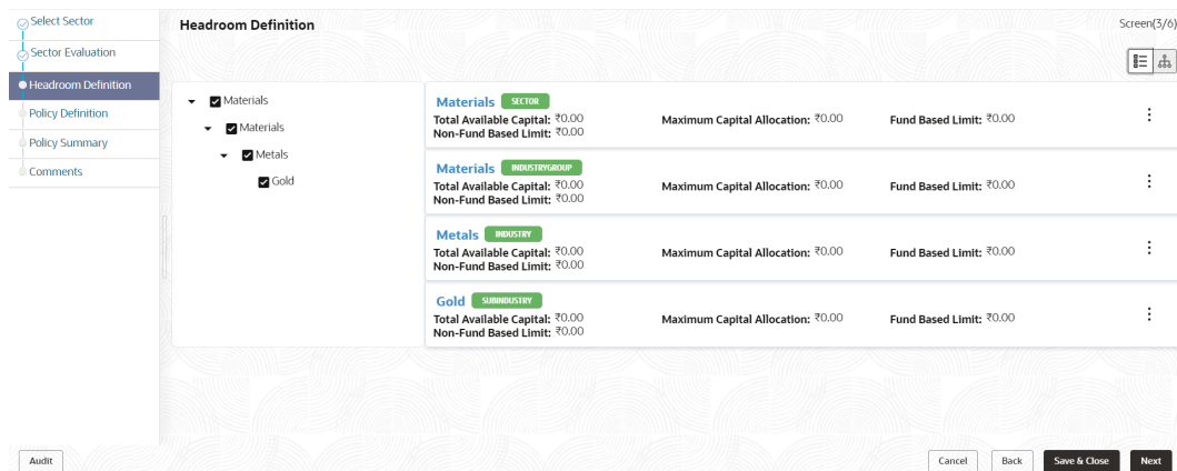
Figure 3-14 Headroom Definition
