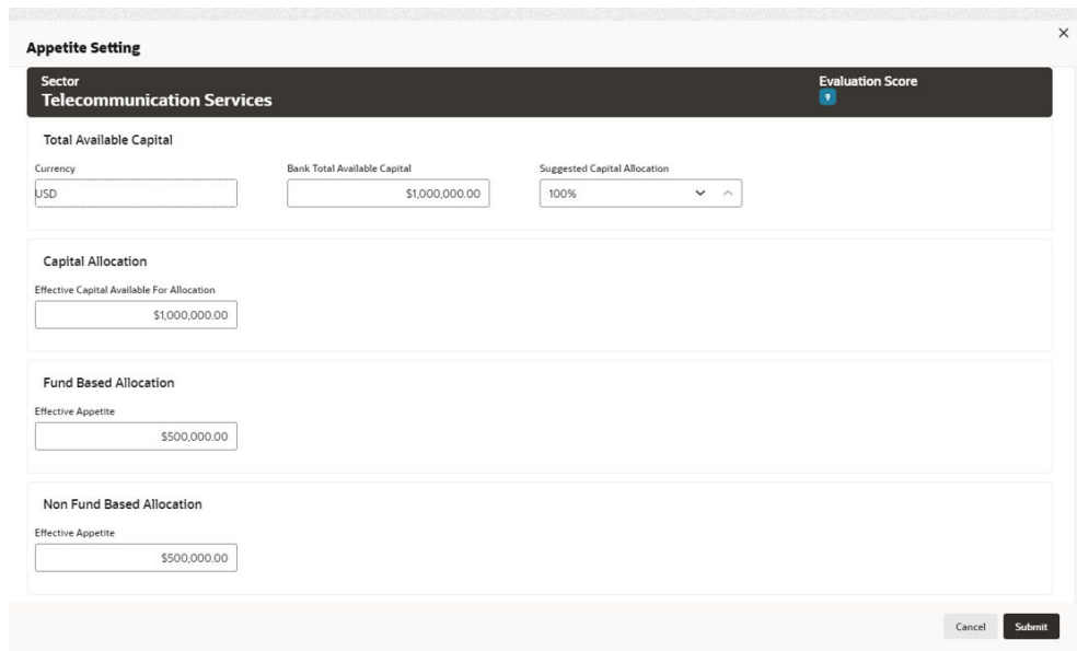
Figure 3-16 Appetite Setting
