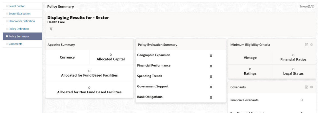
Figure 3-65 Policy Summary
