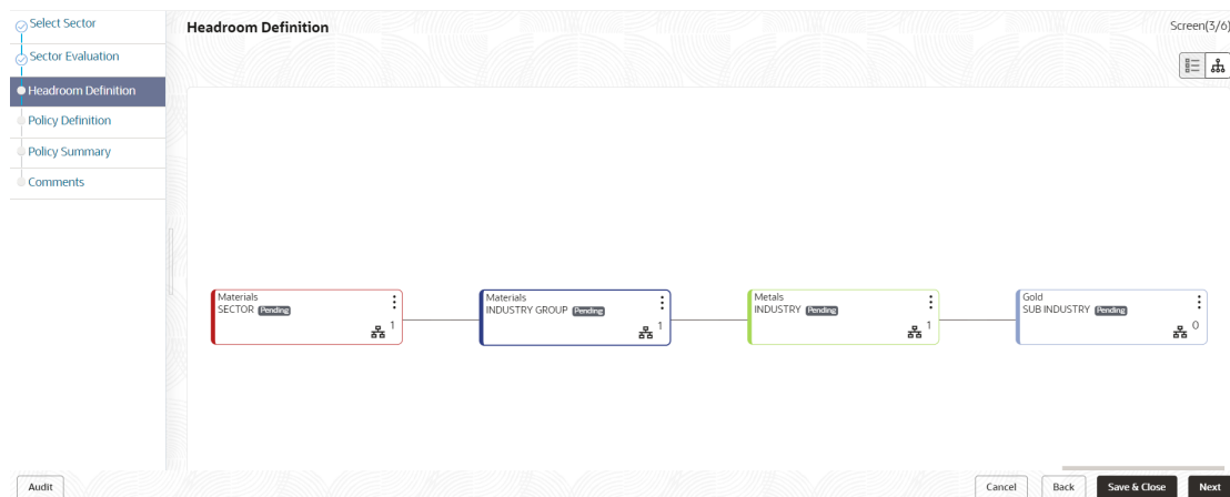
Figure 3-13 Headroom Definition
